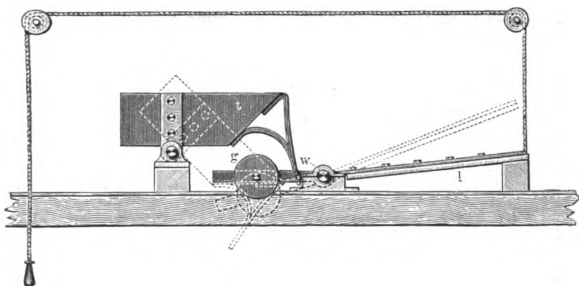
FIG. 93.—One-40th full size.
