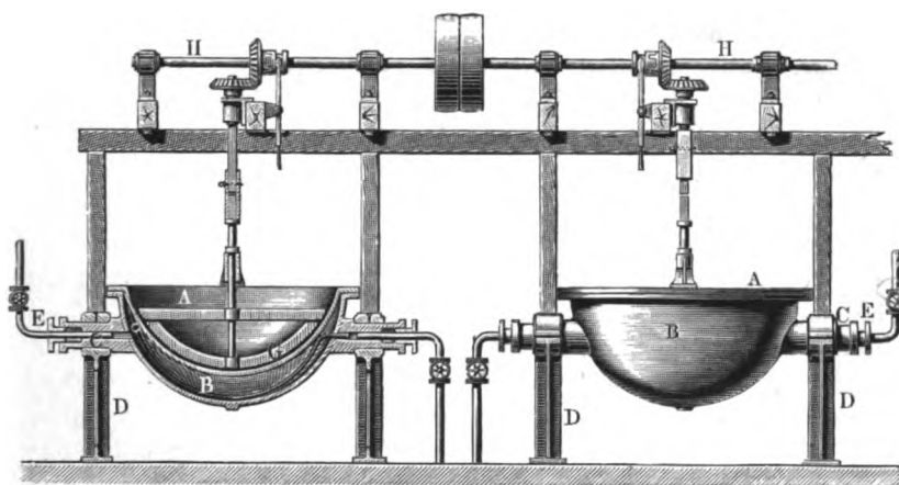
FIG. 136.—One-36th full size.
